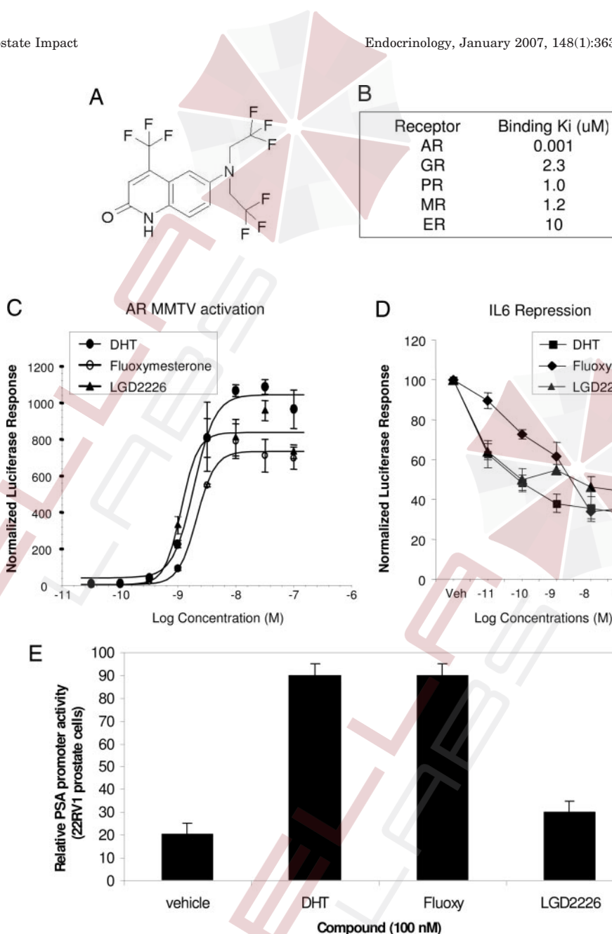
FIG. 1. LGD2226, a selective AR agonist. A and B, The structure (A) of LGD2226 (6-[bis-(2,2,2-trifluoroethyl)amino]-4-trifluoromethyl-1 H -quinolin-2-one) is shown together with a table (B) showing its high-affinity binding for AR and low-affinity binding for other steroid receptors (GR, PR, and MR). C, Cotransfection experiments demonstrating full activation from the MMTV-Luc reporter in response to increasing concentrations of DHT (●), fluoxymesterone (○), and LGD2226 (▲). The SEM is shown for each dose. D, Strong IL-6 repression by DHT (■), fluoxymesterone (◆), and LGD2226 (▲) is shown. The SEM is also plotted for each dose. E, Cotransfection experiments demonstrating partial agonist activity of LGD2226 in a 22RV1 prostate cancer cell line measuring activation of the PSA promoter by the compound compared with steroidal androgens (DHT and fluoxymesterone) at the same dose. Vehicle is used as a background control, and SEM is shown on top of each column with error bars.
