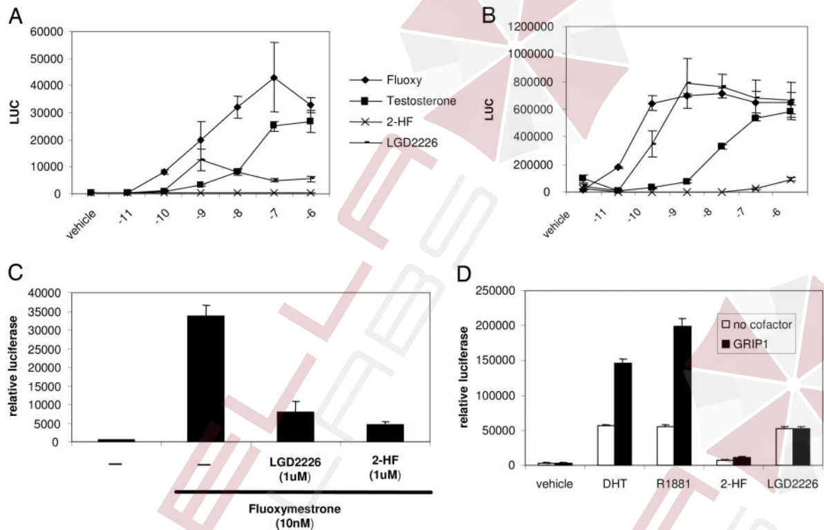
FIG. 2. LGD2226-specific alterations in AR-coactivator interactions. A, HepG2 cells were transfected with plasmids encoding a Gal4-luciferase reporter, Gal4-FxxLF (F-peptide), VPI6-hAR, and RSV- \beta -Gal as a normalization control. After treatment with compounds or reference steroids for 24 h, cells were assayed for luciferase activity. B, Cells were transfected as in A, except that Gal4-D11/F replaced the F-peptide. C, Cells were transfected as in A. Luciferase and \beta -Gal values were determined after 24 h. Cell treatments were 1) vehicle alone, 2) 10 nM fluoxymesterone, 3) 10 nM fluoxymesterone and 1 \mu M LGD2226, and 4) 10 nM fluoxymesterone and 1 \mu M 2-hydroxyflutamide. D, CV-1 cells were transfected with AR, MMTV-Luc reporter, RSV- \beta -Gal, and pSG5-HA.GRIP1. After 24 h, the cells were treated with the different compounds for 24 h at 10 \mu M. Assays were done as for A.
